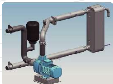
Hydraulic module (additional option)
